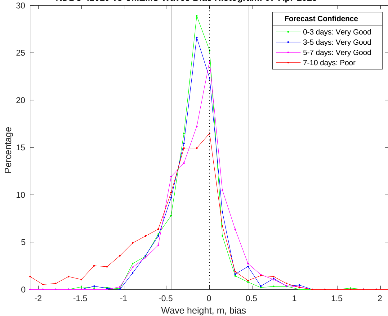
NDBC 42019 vs CMEMS Waves Bias Histogram: 07-Apr-2025
