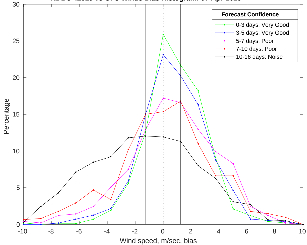
NDBC 42019 vs GFS Winds Bias Histogram: 07-Apr-2025
