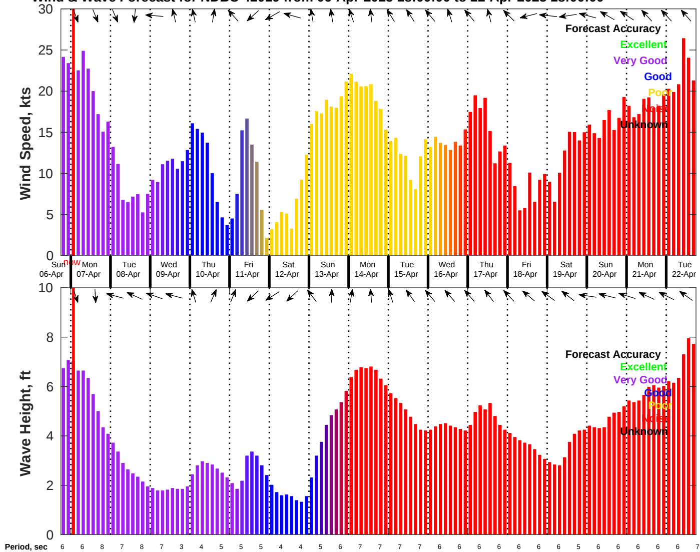
Wind & Wave Forecast for NDBC 42019 from 06-Apr-2025 18:00:00 to 22-Apr-2025 18:00:00
