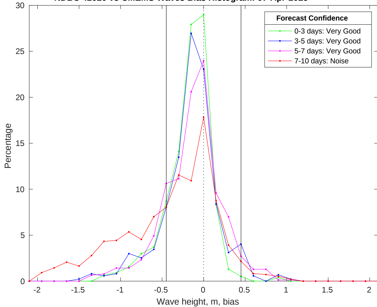
NDBC 42020 vs CMEMS Waves Bias Histogram: 07-Apr-2025
