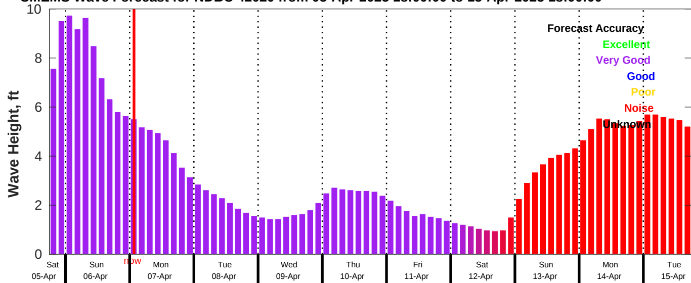
CMEMS Wave Forecast for NDBC 42020 from 05-Apr-2025 18:00:00 to 15-Apr-2025 18:00:00
