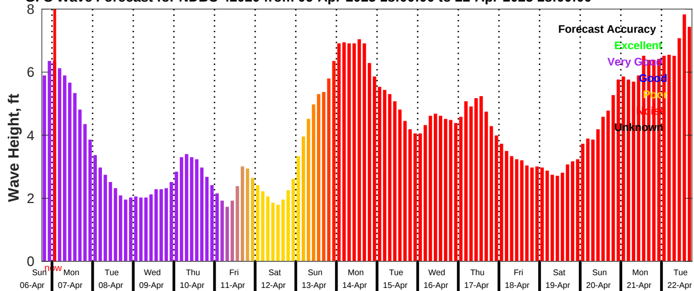
GFS Wave Forecast for NDBC 42020 from 06-Apr-2025 18:00:00 to 22-Apr-2025 18:00:00
