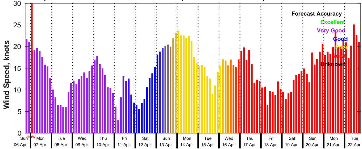
GFS Wind Speed Forecast for NDBC 42020 from 06-Apr-2025 18:00:00 to 22-Apr-2025 18:00:00
