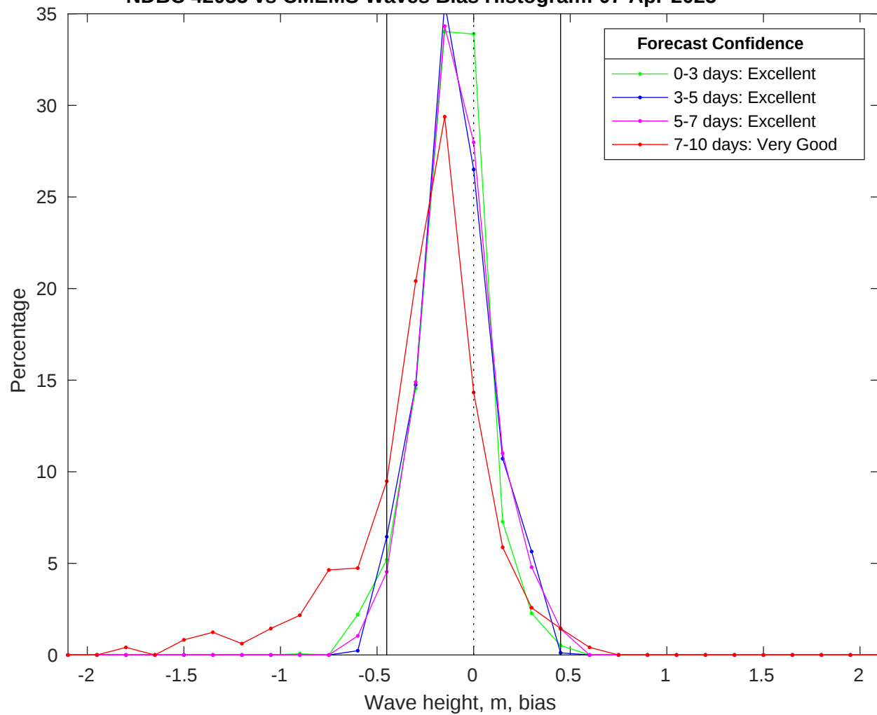
NDBC 42035 vs CMEMS Waves Bias Histogram: 07-Apr-2025
