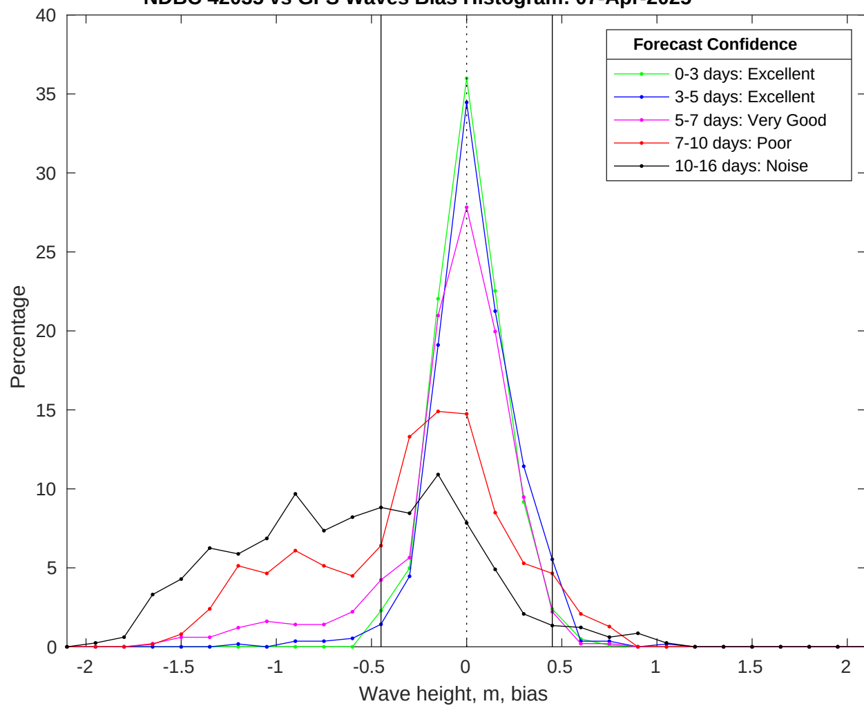
NDBC 42035 vs GFS Waves Bias Histogram: 07-Apr-2025
