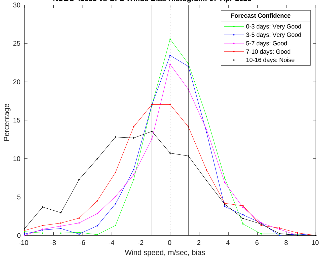
NDBC 42035 vs GFS Winds Bias Histogram: 07-Apr-2025
