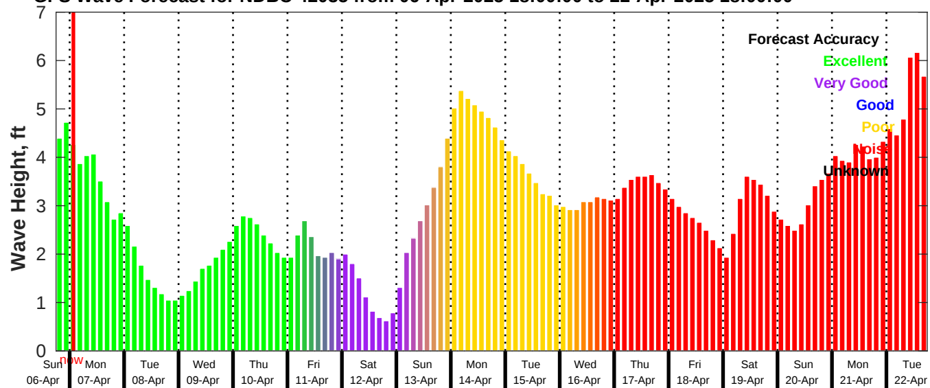
GFS Wave Forecast for NDBC 42035 from 06-Apr-2025 18:00:00 to 22-Apr-2025 18:00:00
