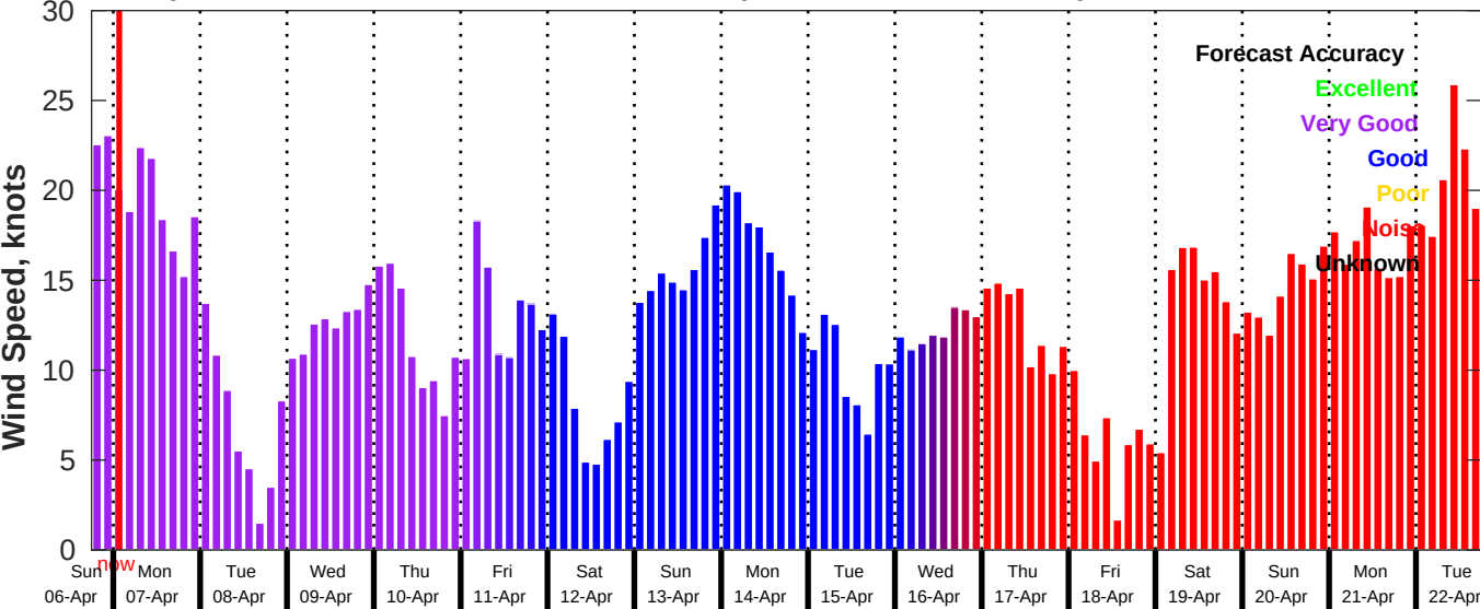
GFS Wind Speed Forecast for NDBC 42035 from 06-Apr-2025 18:00:00 to 22-Apr-2025 18:00:00
