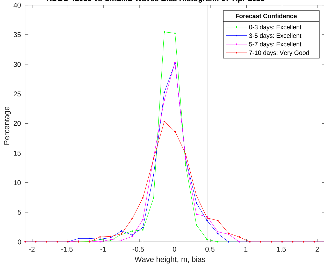
NDBC 42036 vs CMEMS Waves Bias Histogram: 07-Apr-2025
