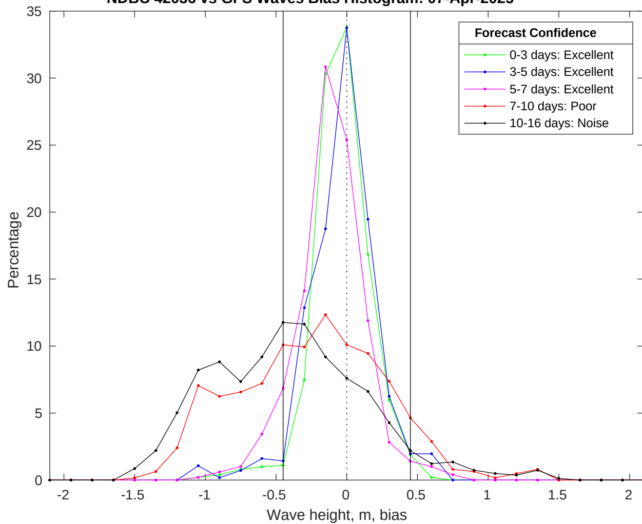
NDBC 42036 vs GFS Waves Bias Histogram: 07-Apr-2025
