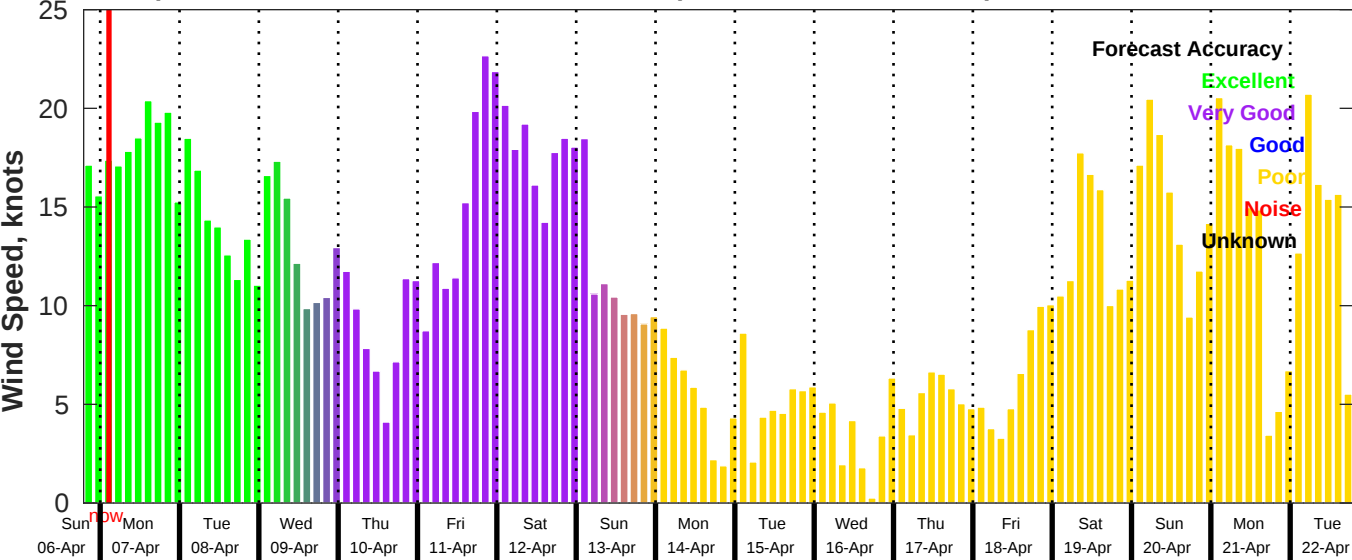
GFS Wind Speed Forecast for NDBC 42036 from 06-Apr-2025 19:00:00 to 22-Apr-2025 19:00:00
