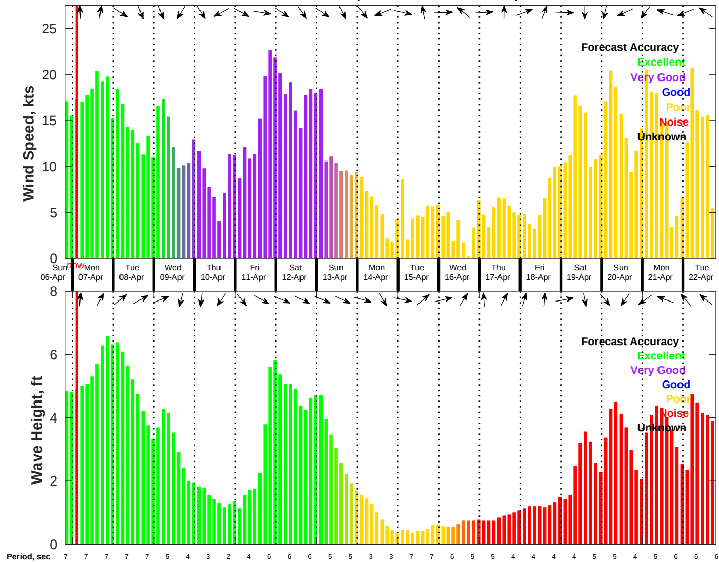
Wind & Wave Forecast for NDBC 42036 from 06-Apr-2025 19:00:00 to 22-Apr-2025 19:00:00
