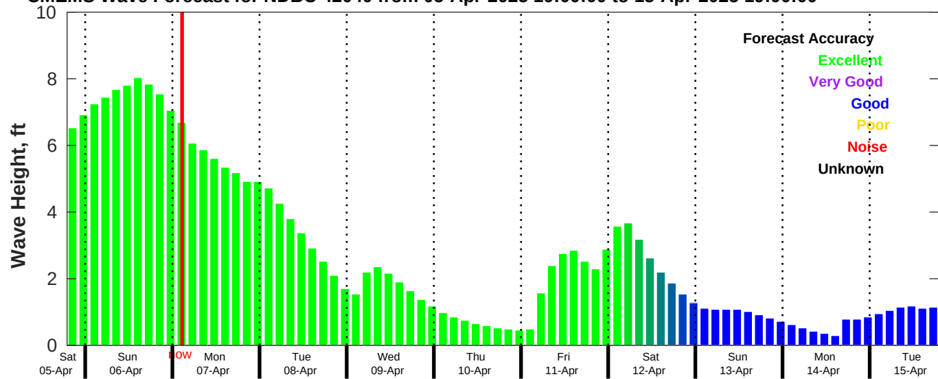
CMEMS Wave Forecast for NDBC 42040 from 05-Apr-2025 19:00:00 to 15-Apr-2025 19:00:00
