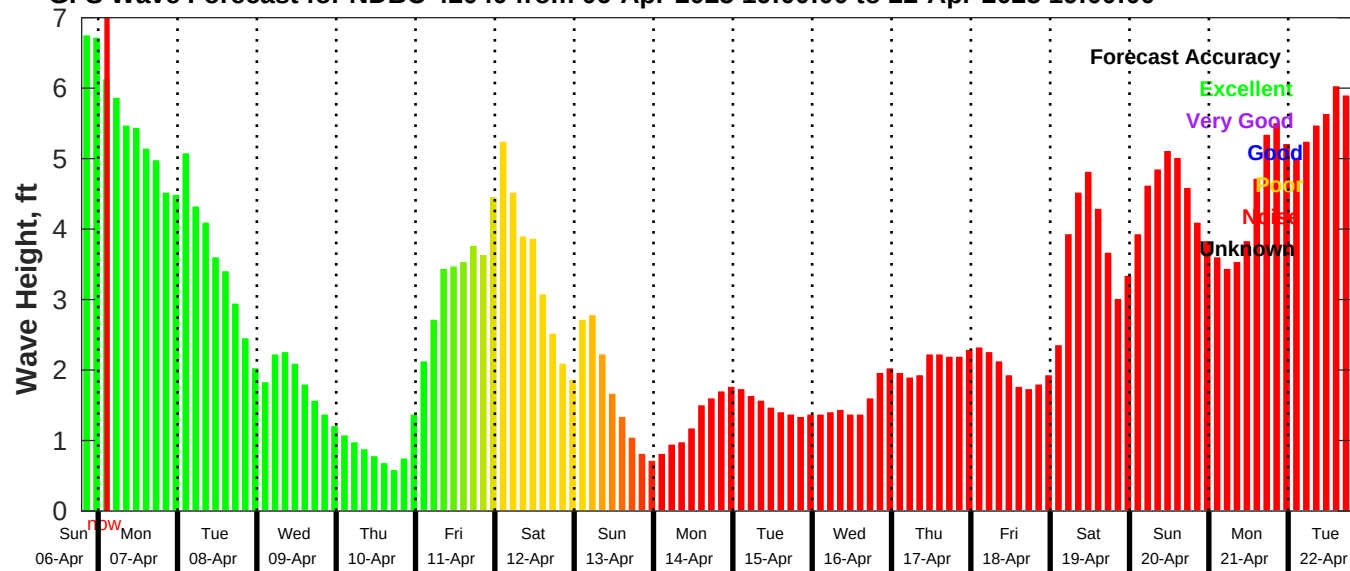
GFS Wave Forecast for NDBC 42040 from 06-Apr-2025 19:00:00 to 22-Apr-2025 19:00:00
