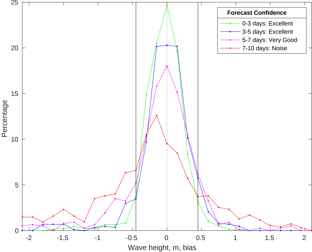
NDBC 46011 vs CMEMS Waves Bias Histogram: 07-Apr-2025
