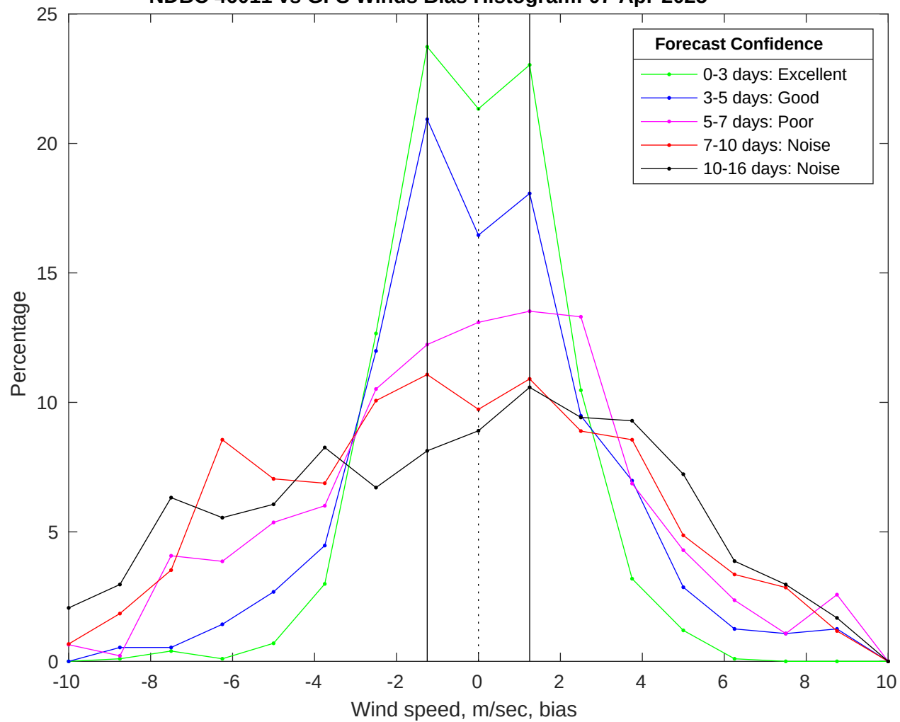
NDBC 46011 vs GFS Winds Bias Histogram: 07-Apr-2025
