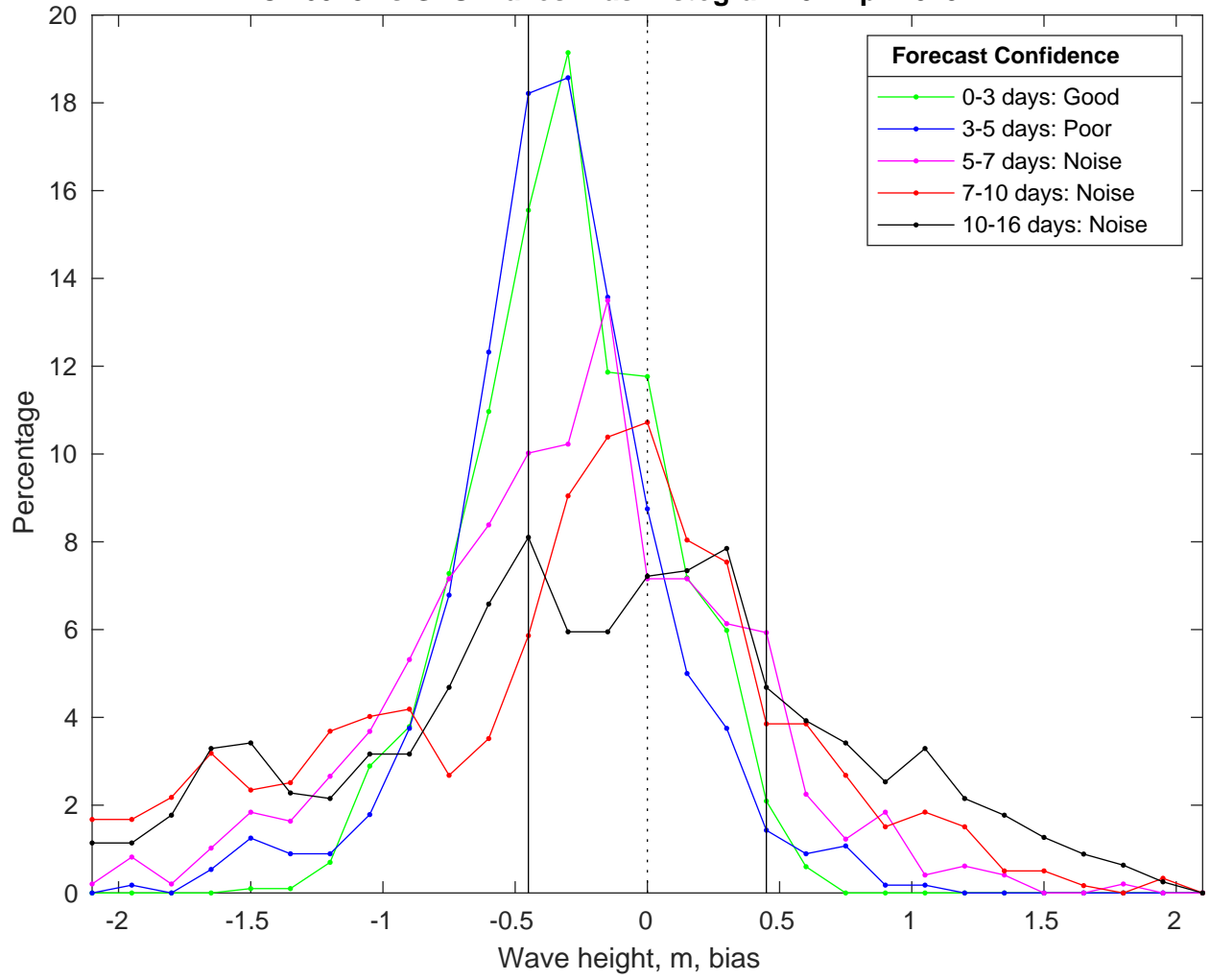
NDBC 46028 vs GFS Waves Bias Histogram: 07-Apr-2025
