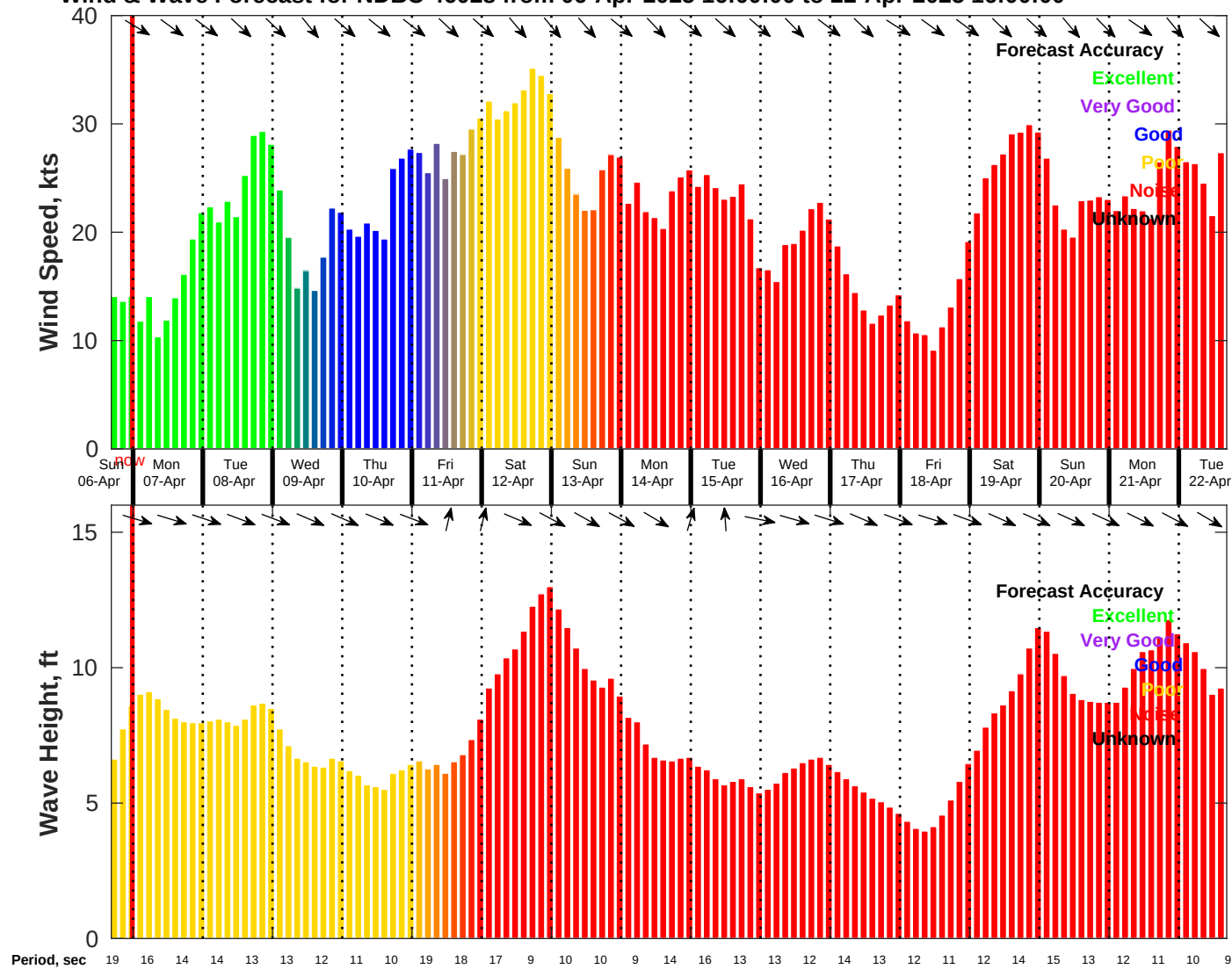
Wind & Wave Forecast for NDBC 46028 from 06-Apr-2025 16:00:00 to 22-Apr-2025 16:00:00
