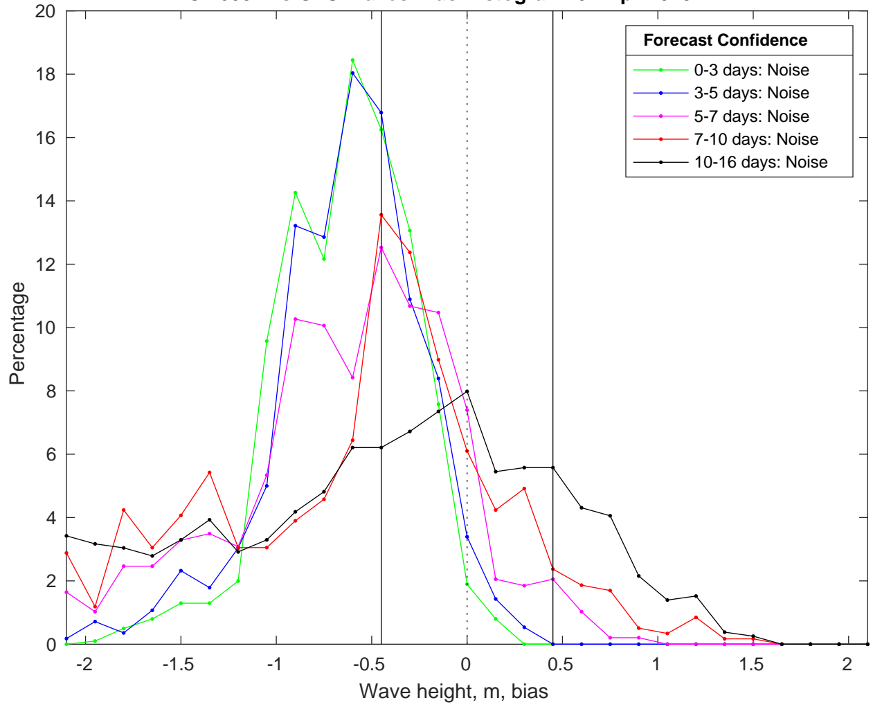
NDBC 46054 vs GFS Waves Bias Histogram: 07-Apr-2025
