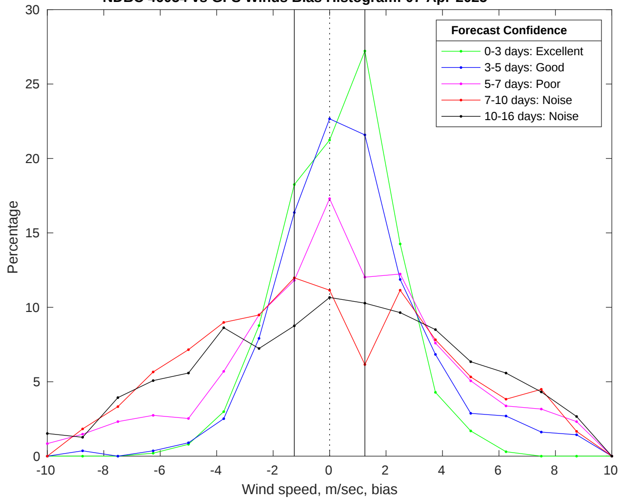
NDBC 46054 vs GFS Winds Bias Histogram: 07-Apr-2025
