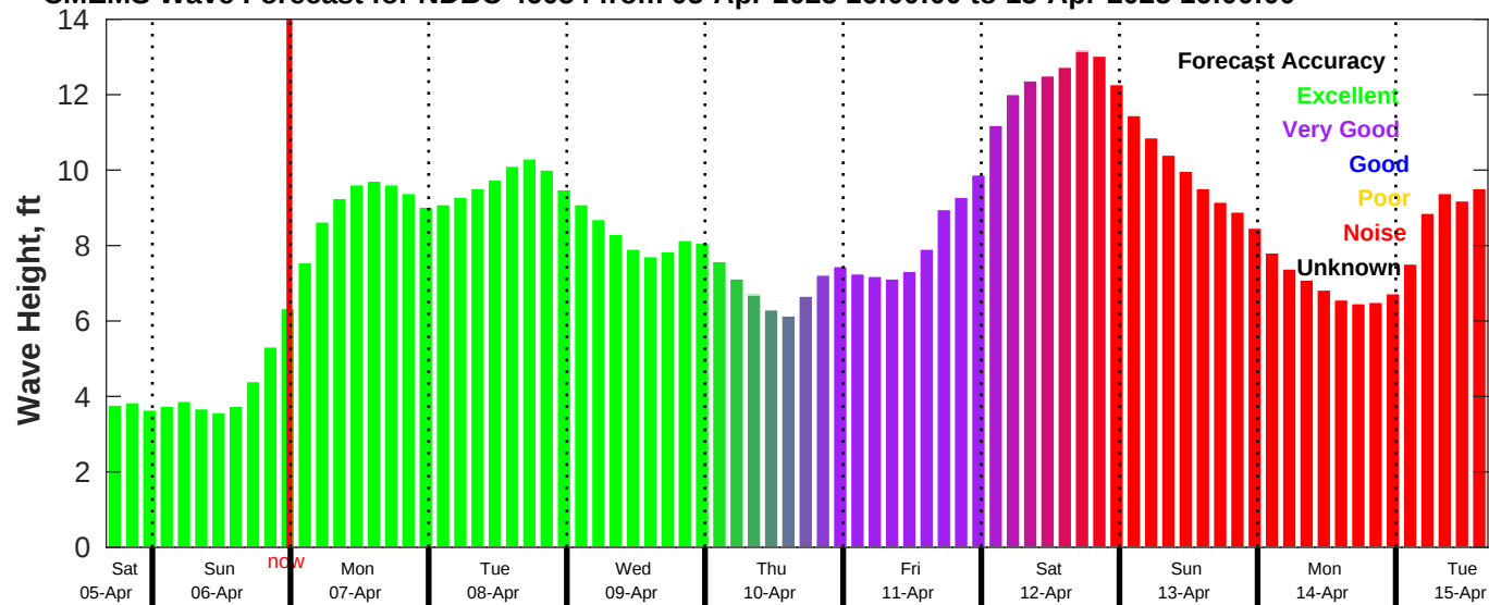
CMEMS Wave Forecast for NDBC 46054 from 05-Apr-2025 16:00:00 to 15-Apr-2025 16:00:00
