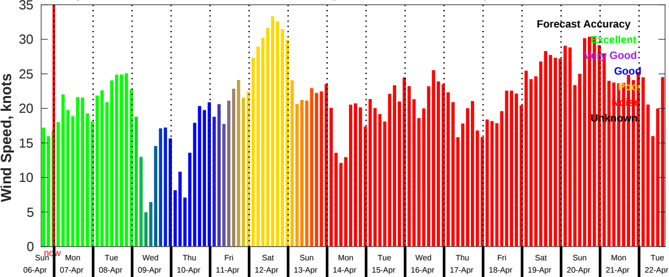
GFS Wind Speed Forecast for NDBC 46054 from 06-Apr-2025 16:00:00 to 22-Apr-2025 16:00:00
