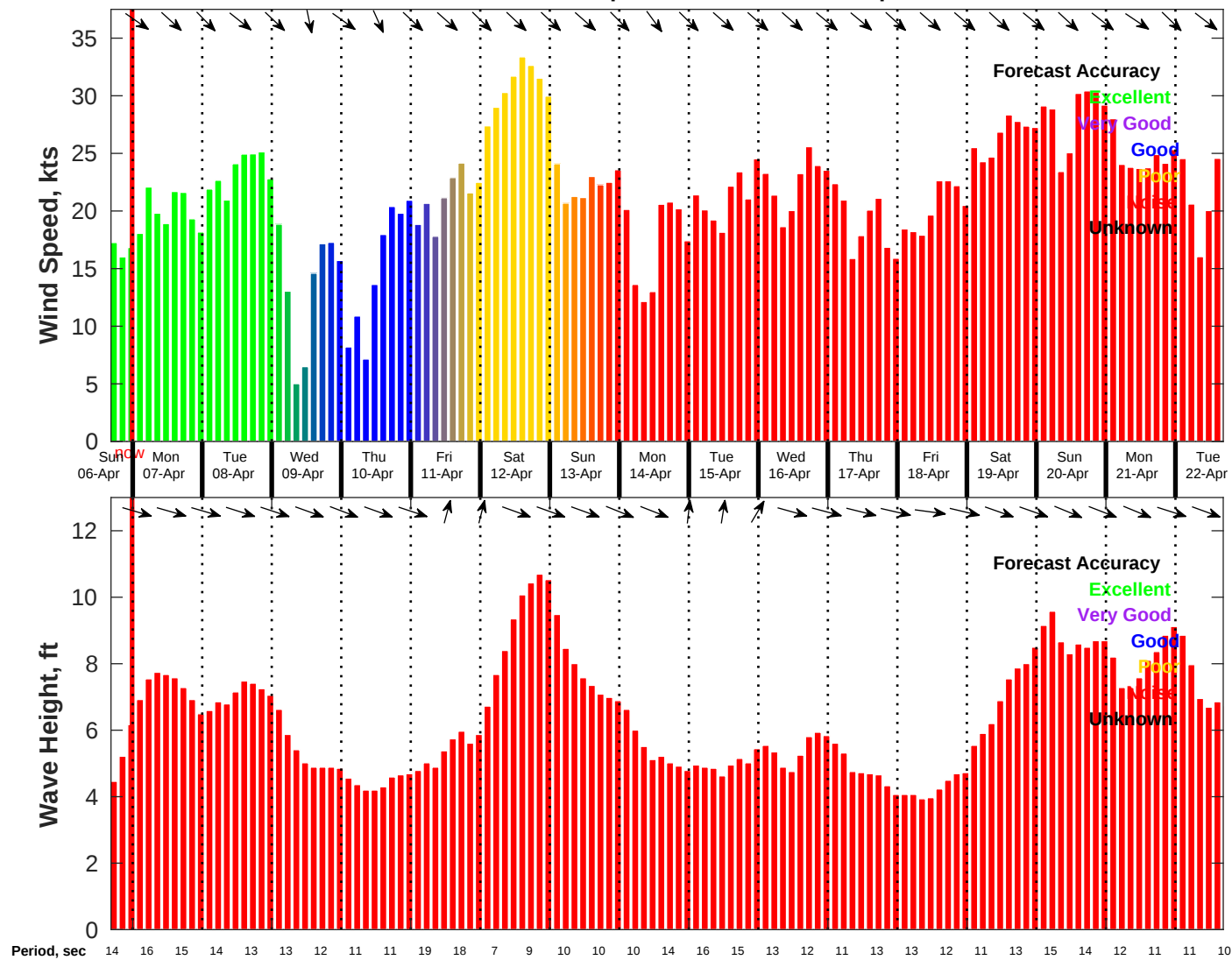
Wind & Wave Forecast for NDBC 46054 from 06-Apr-2025 16:00:00 to 22-Apr-2025 16:00:00
