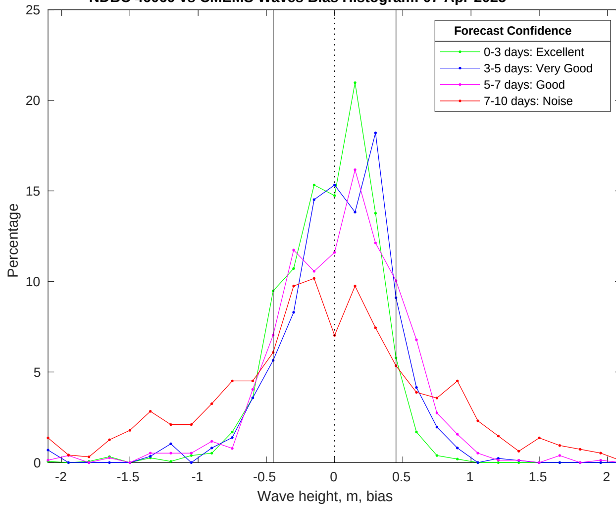
NDBC 46069 vs CMEMS Waves Bias Histogram: 07-Apr-2025
