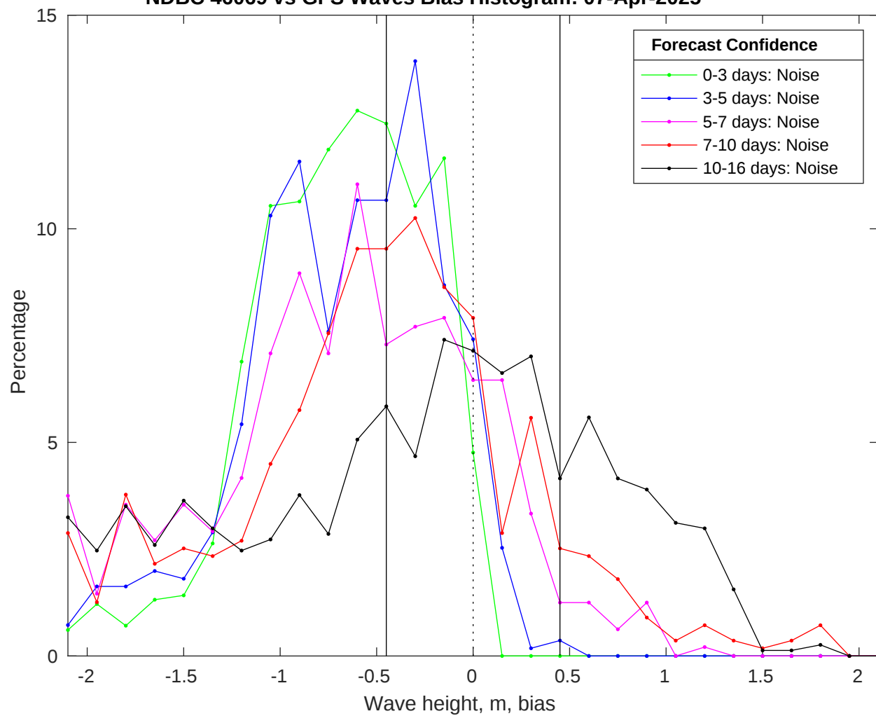
NDBC 46069 vs GFS Waves Bias Histogram: 07-Apr-2025
