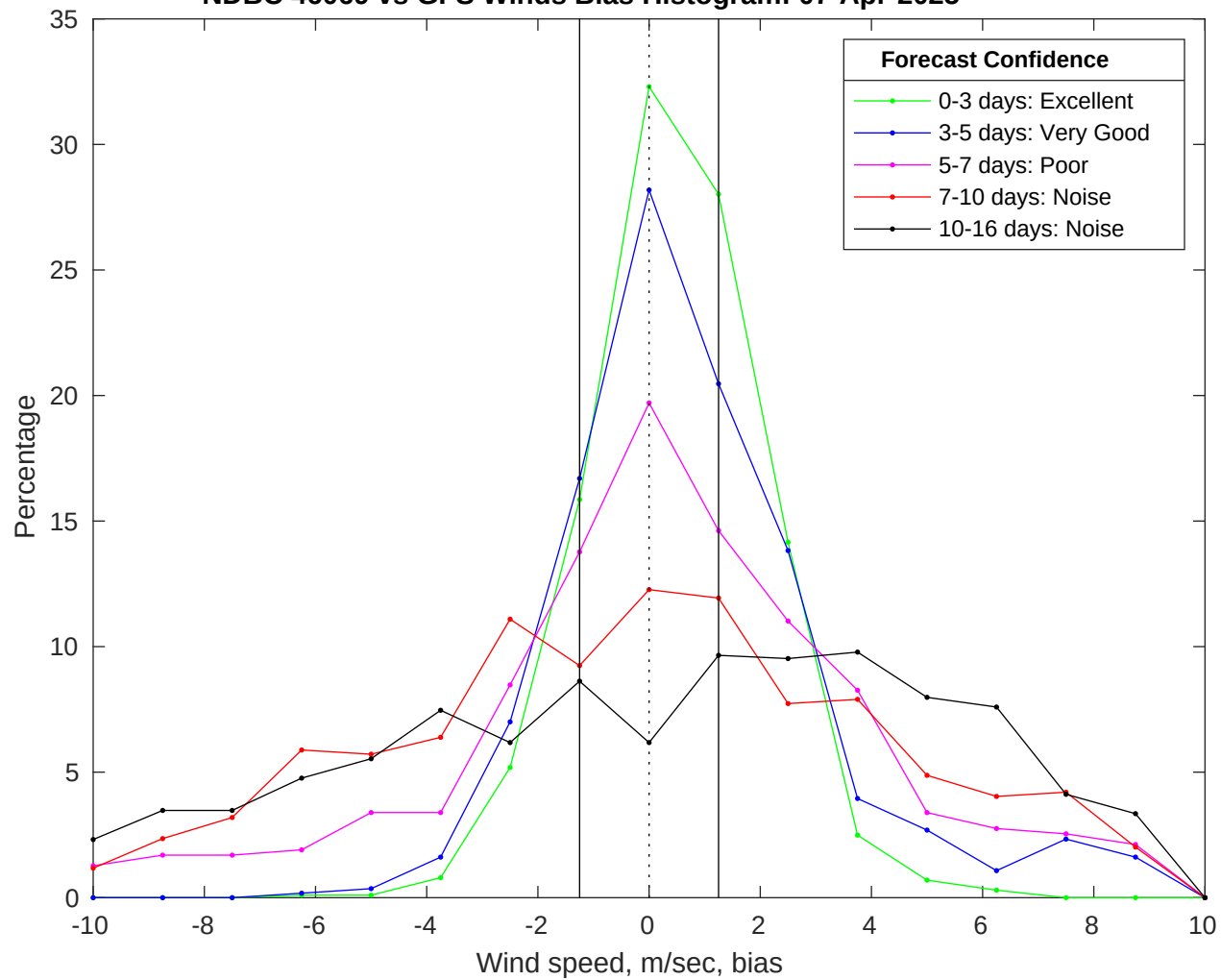
NDBC 46069 vs GFS Winds Bias Histogram: 07-Apr-2025
