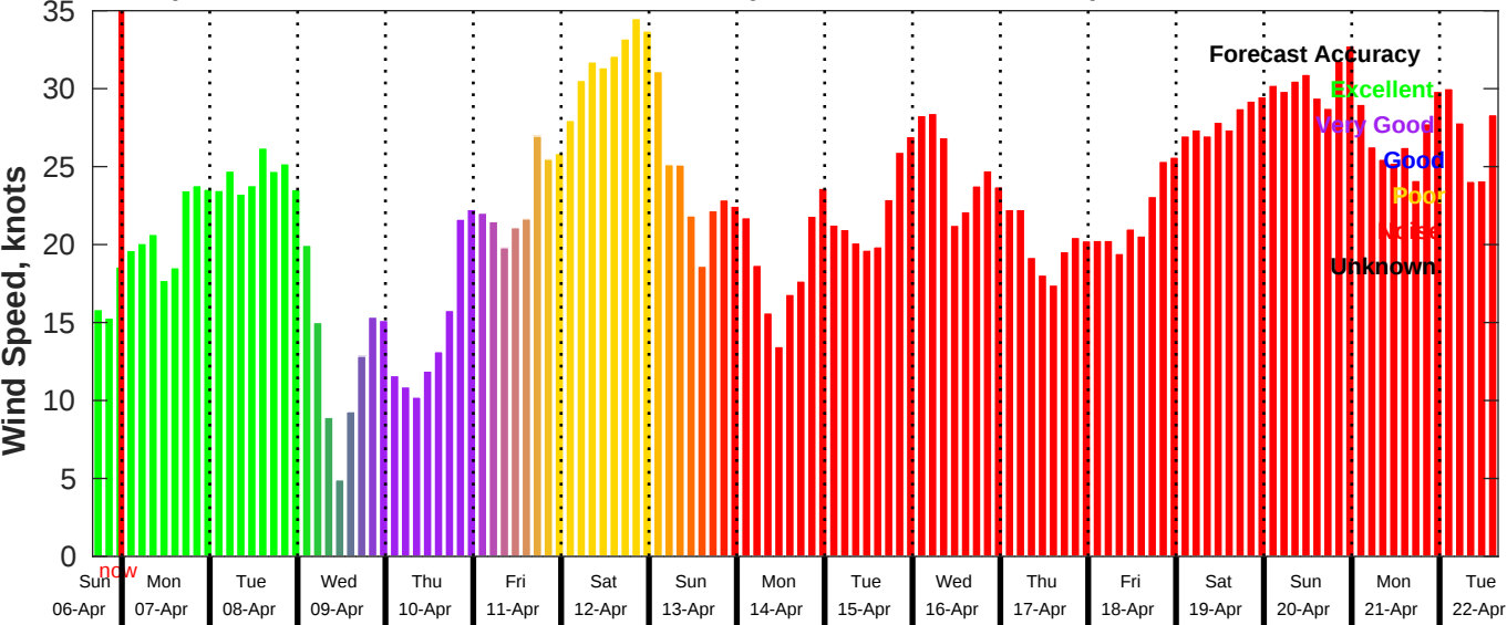
GFS Wind Speed Forecast for NDBC 46069 from 06-Apr-2025 16:00:00 to 22-Apr-2025 16:00:00
