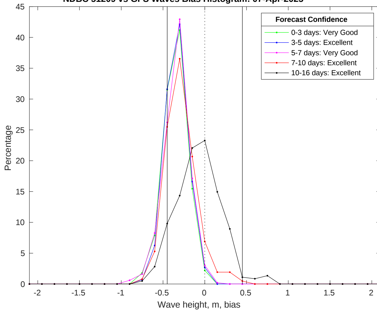
NDBC 51209 vs GFS Waves Bias Histogram: 07-Apr-2025
