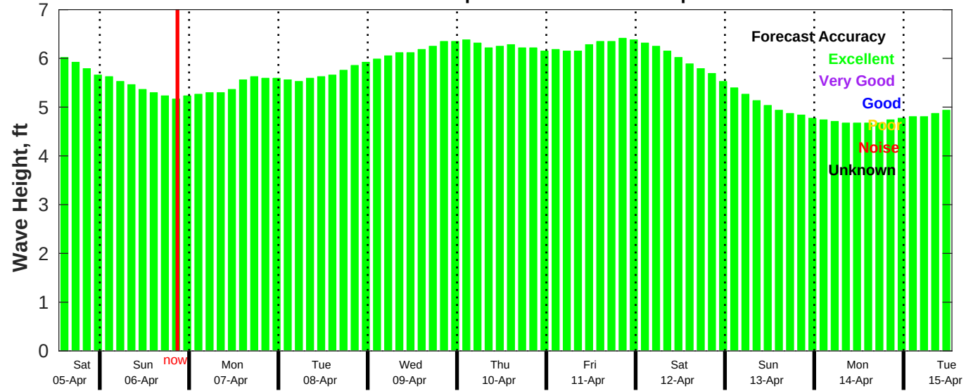
CMEMS Wave Forecast for NDBC 51209 from 05-Apr-2025 13:00:00 to 15-Apr-2025 13:00:00
