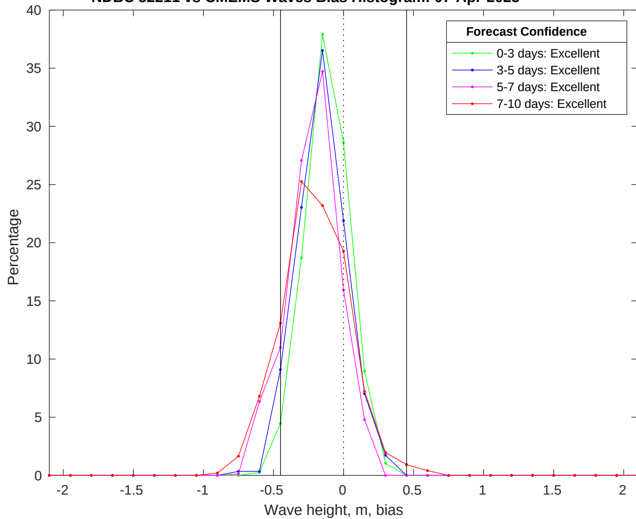
NDBC 52211 vs CMEMS Waves Bias Histogram: 07-Apr-2025
