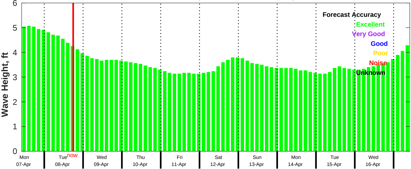
CMEMS Wave Forecast for NDBC 52211 from 06-Apr-2025 10:00:00 to 16-Apr-2025 10:00:00
