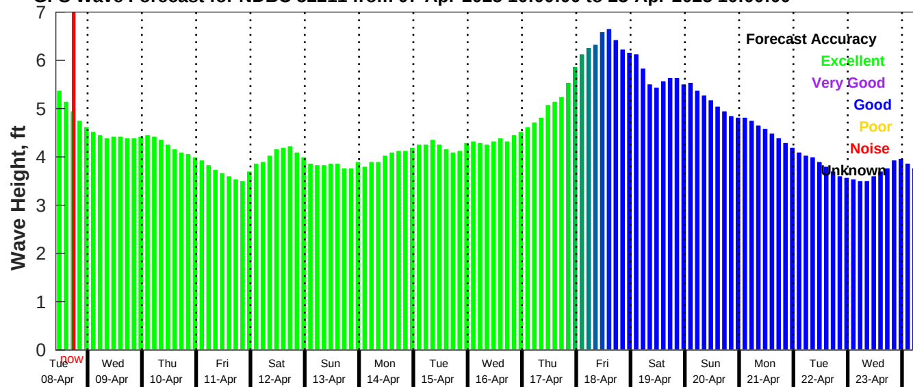
GFS Wave Forecast for NDBC 52211 from 07-Apr-2025 10:00:00 to 23-Apr-2025 10:00:00
