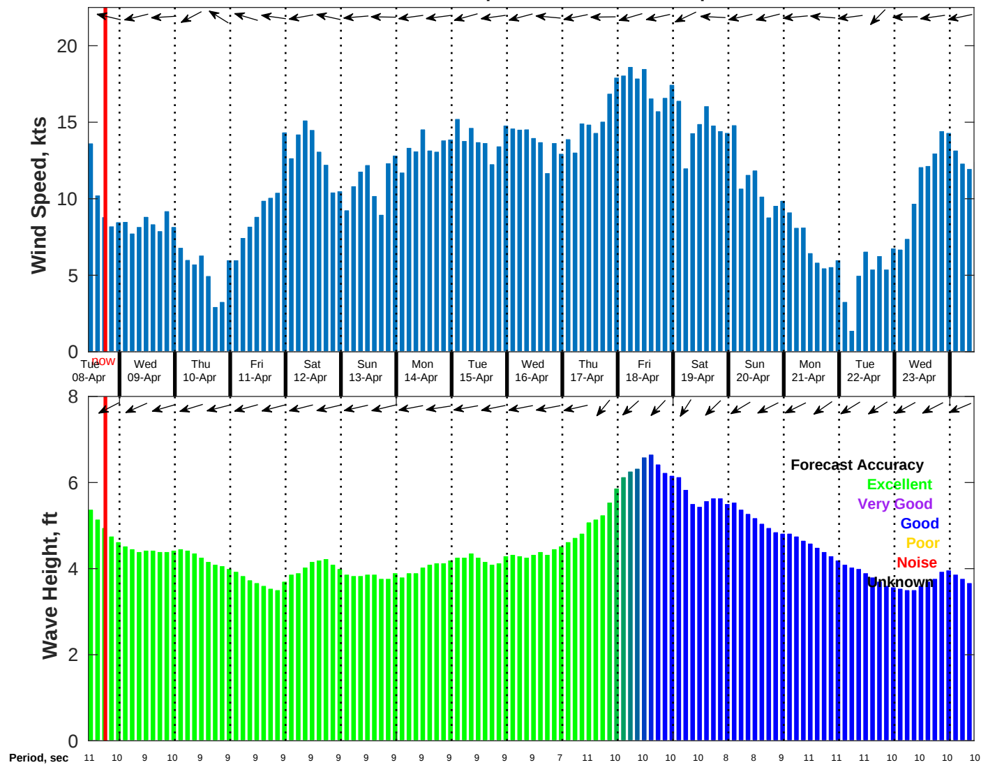
Wind & Wave Forecast for NDBC 52211 from 07-Apr-2025 10:00:00 to 23-Apr-2025 10:00:00
