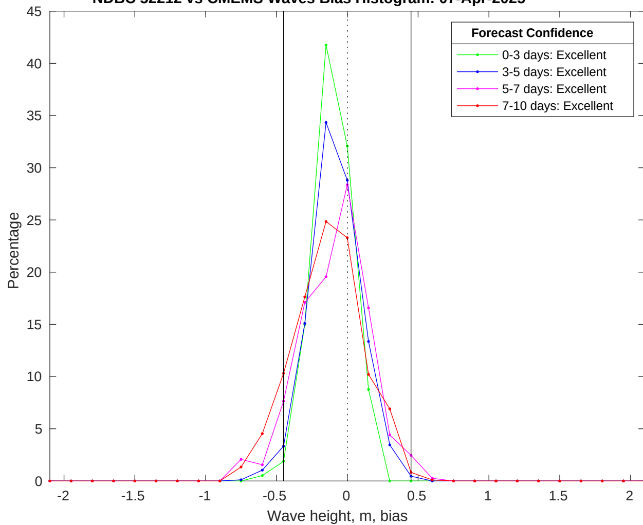
NDBC 52212 vs CMEMS Waves Bias Histogram: 07-Apr-2025
