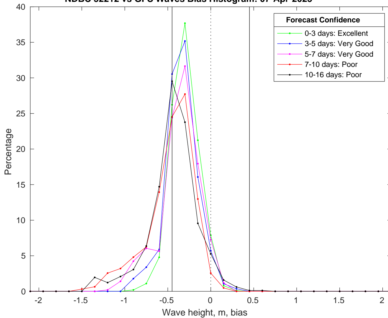
NDBC 52212 vs GFS Waves Bias Histogram: 07-Apr-2025
