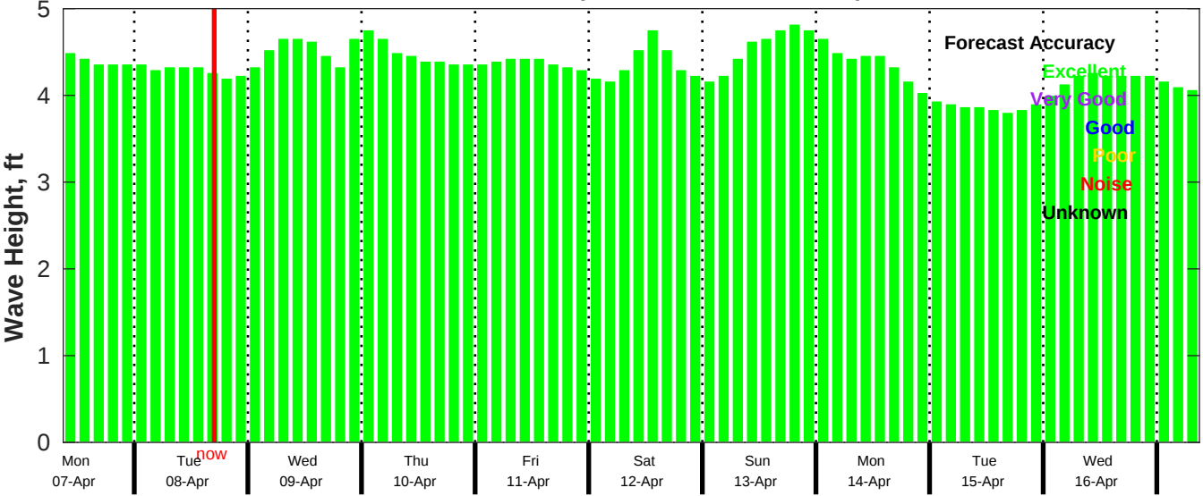
CMEMS Wave Forecast for NDBC 52212 from 06-Apr-2025 09:00:00 to 16-Apr-2025 09:00:00
