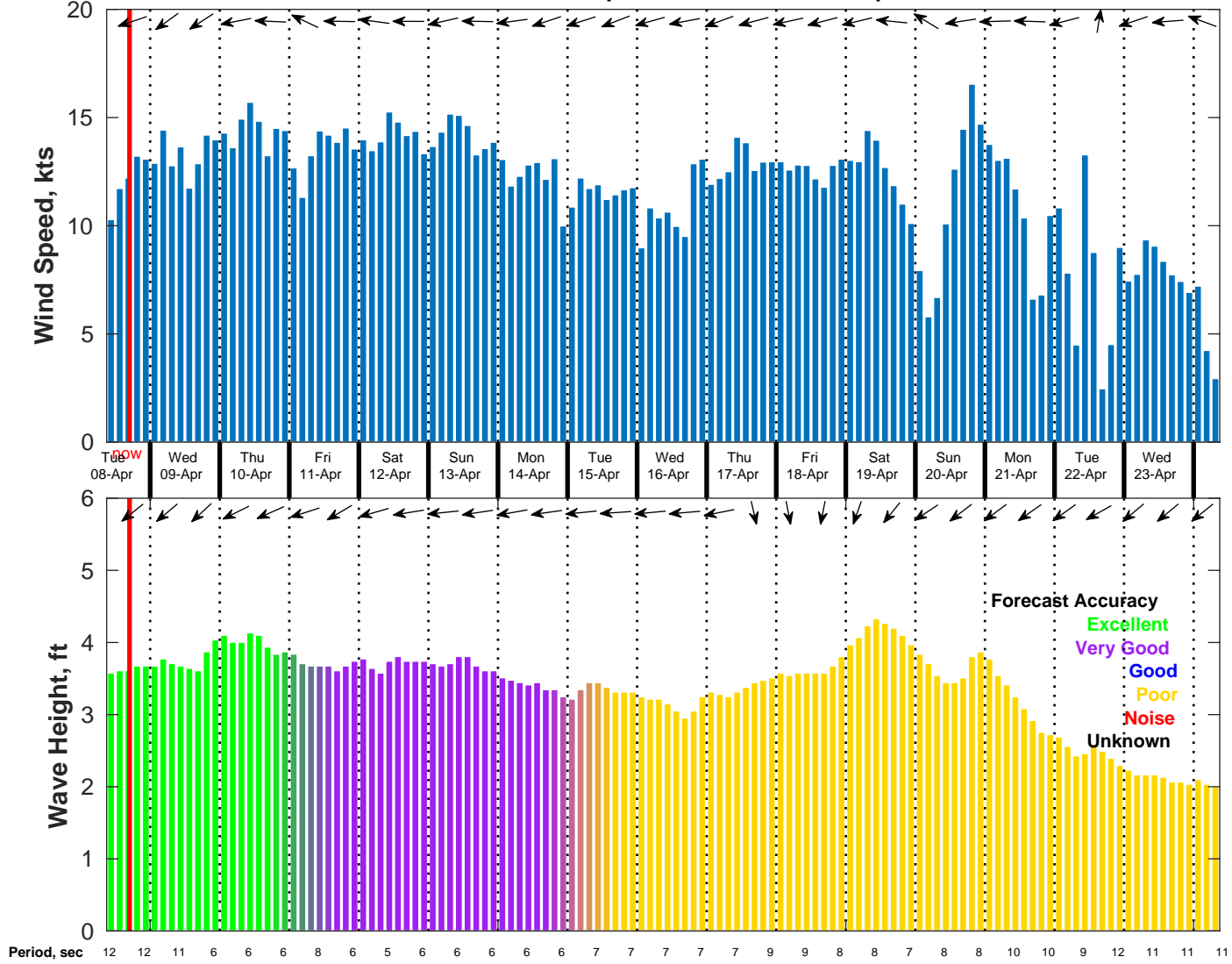
Wind & Wave Forecast for NDBC 52212 from 07-Apr-2025 09:00:00 to 23-Apr-2025 09:00:00
