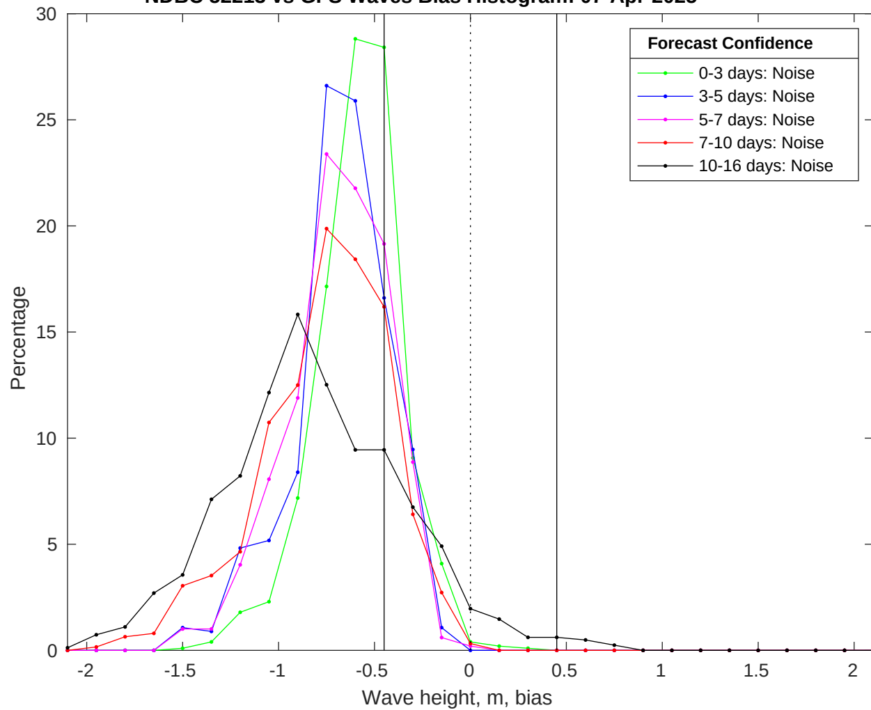
NDBC 52213 vs GFS Waves Bias Histogram: 07-Apr-2025
