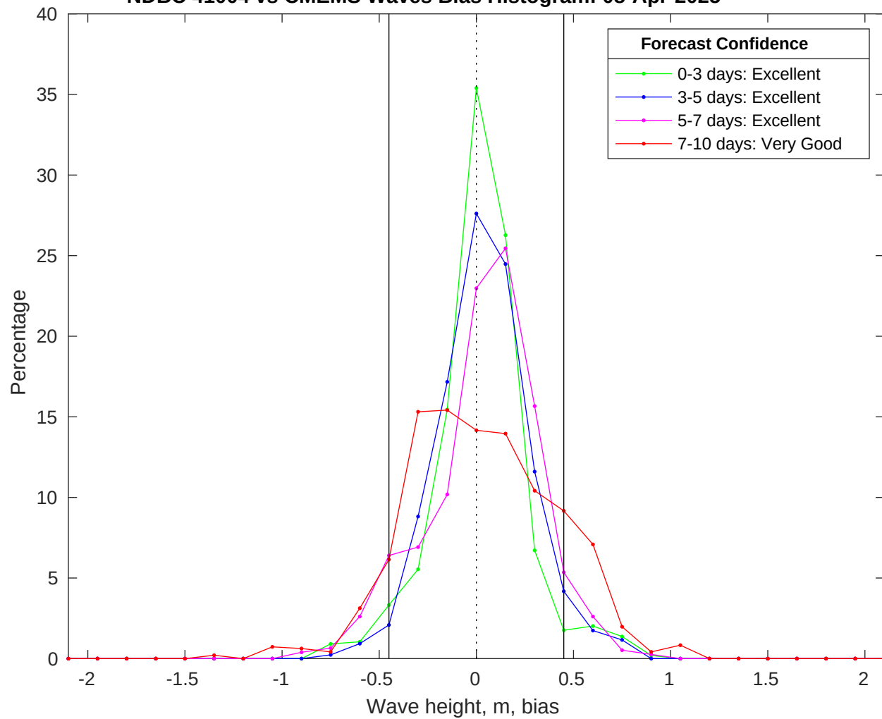
NDBC 41004 vs CMEMS Waves Bias Histogram: 08-Apr-2025
