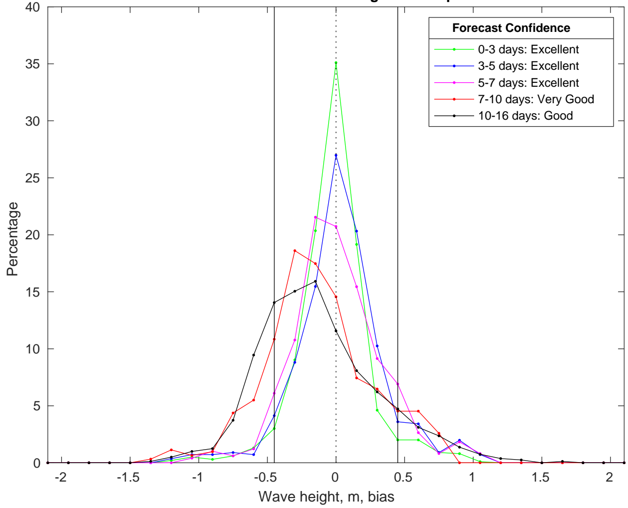
NDBC 41004 vs GFS Waves Bias Histogram: 08-Apr-2025
