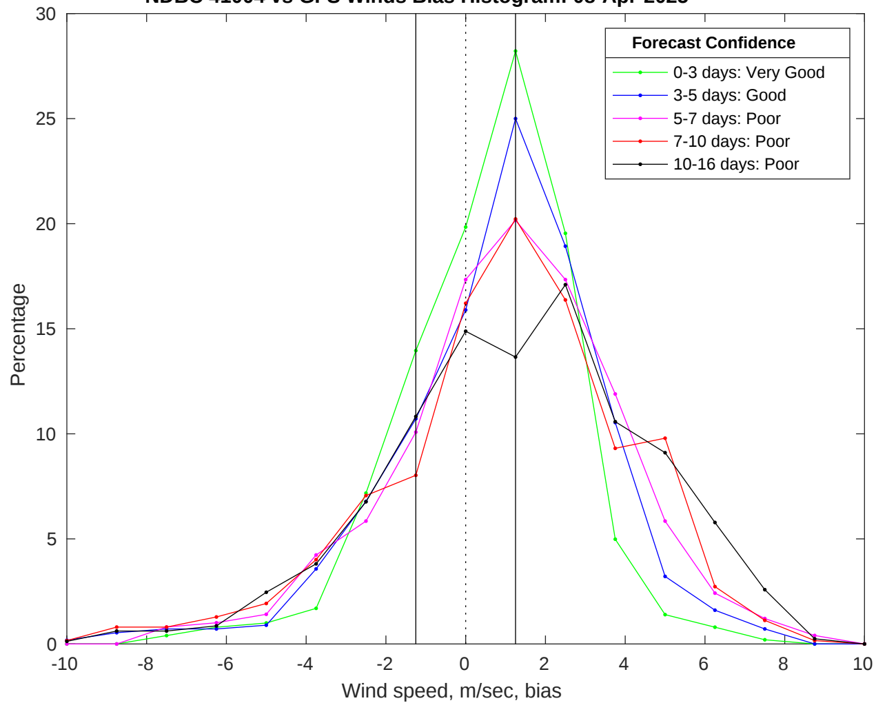
NDBC 41004 vs GFS Winds Bias Histogram: 08-Apr-2025
