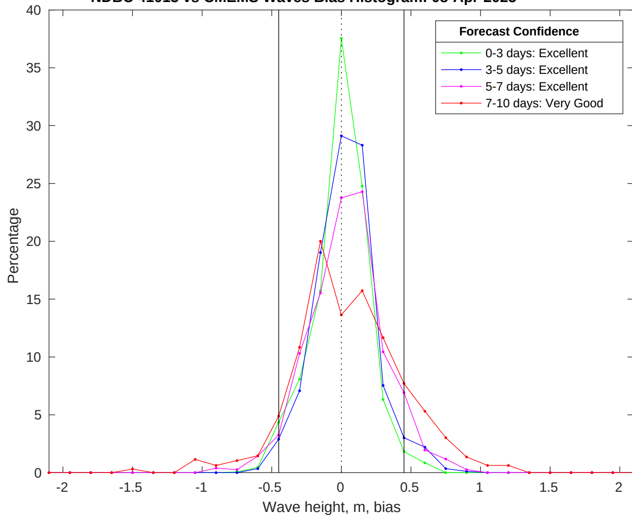
NDBC 41013 vs CMEMS Waves Bias Histogram: 08-Apr-2025
