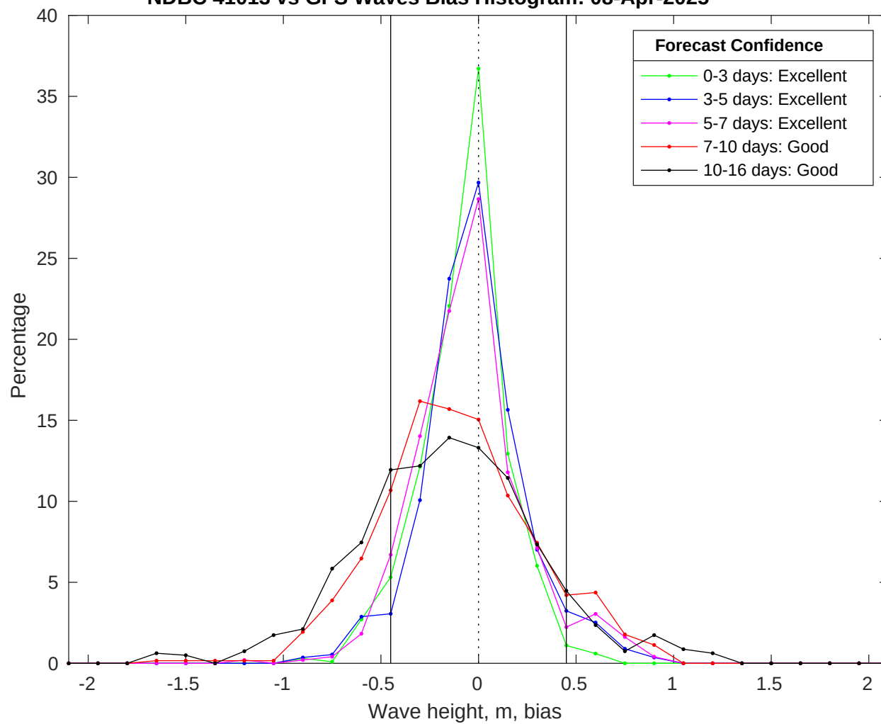
NDBC 41013 vs GFS Waves Bias Histogram: 08-Apr-2025
