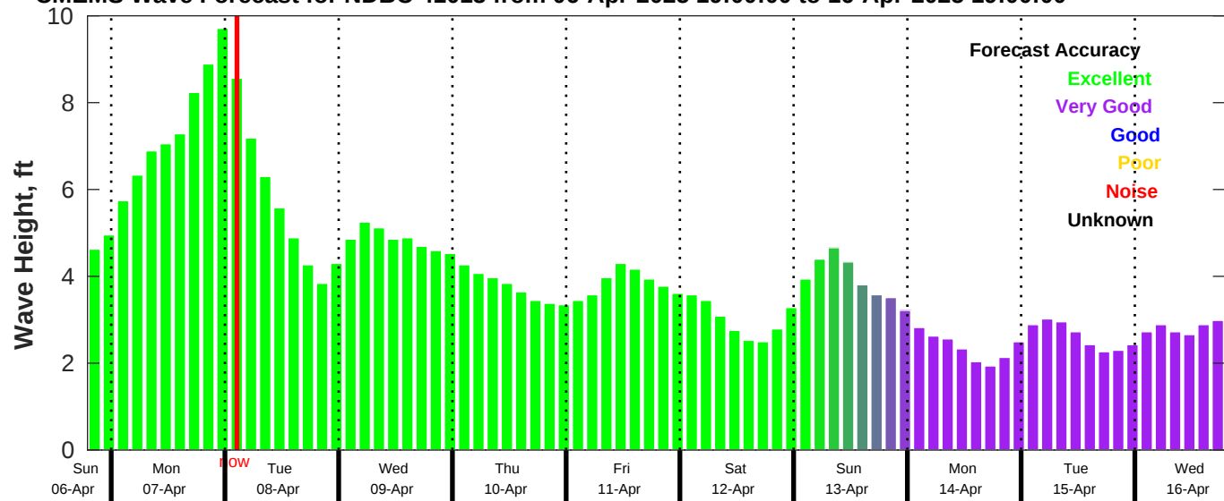
CMEMS Wave Forecast for NDBC 41013 from 06-Apr-2025 19:00:00 to 16-Apr-2025 19:00:00
