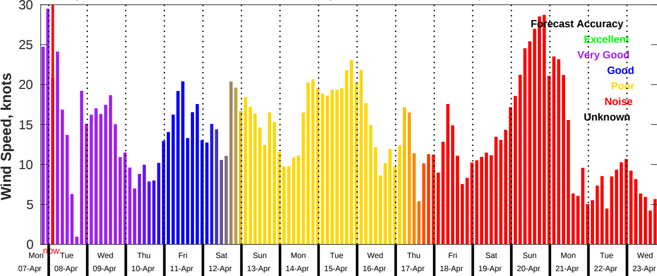
GFS Wind Speed Forecast for NDBC 41013 from 07-Apr-2025 19:00:00 to 23-Apr-2025 19:00:00
