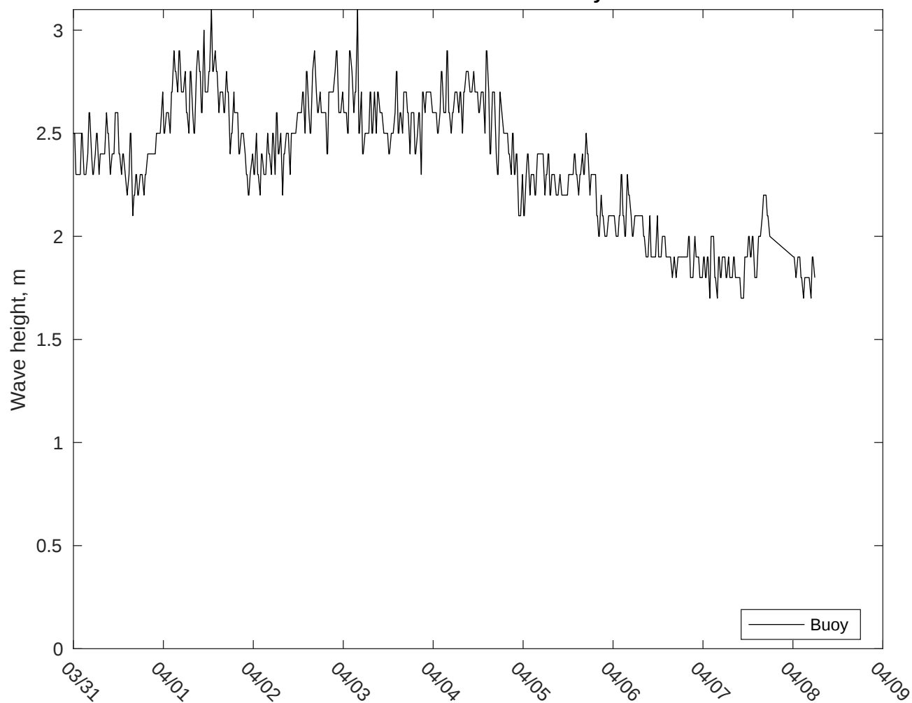
NDBC 41040 vs CMEMS Waves: 10 to 16 day forecast
